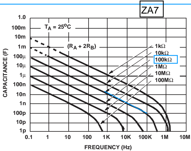
FIGURE 14. FREE RUNNING FREQUENCY vs R_A , R_B AND C
