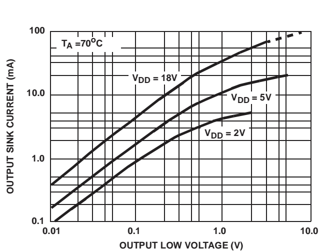
FIGURE 7. OUTPUT SINK CURRENT vs OUTPUT VOLTAGE
