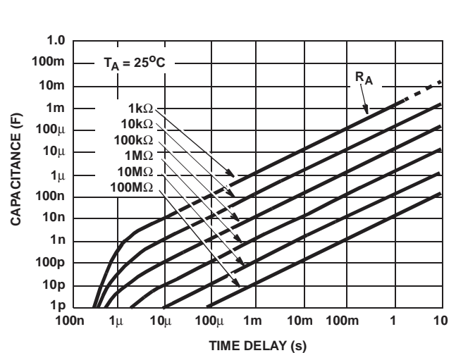
FIGURE 15. TIME DELAY IN THE MONOSTABLE MODE vs R_A AND C
